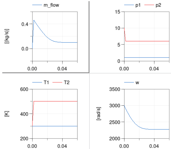
Figure 4: Results of the compressor test model.
